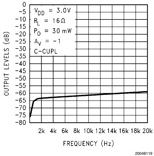
Channel Separation
