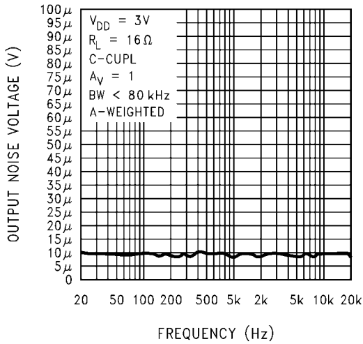
Noise Floor
