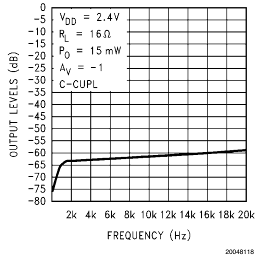
Channel Separation
